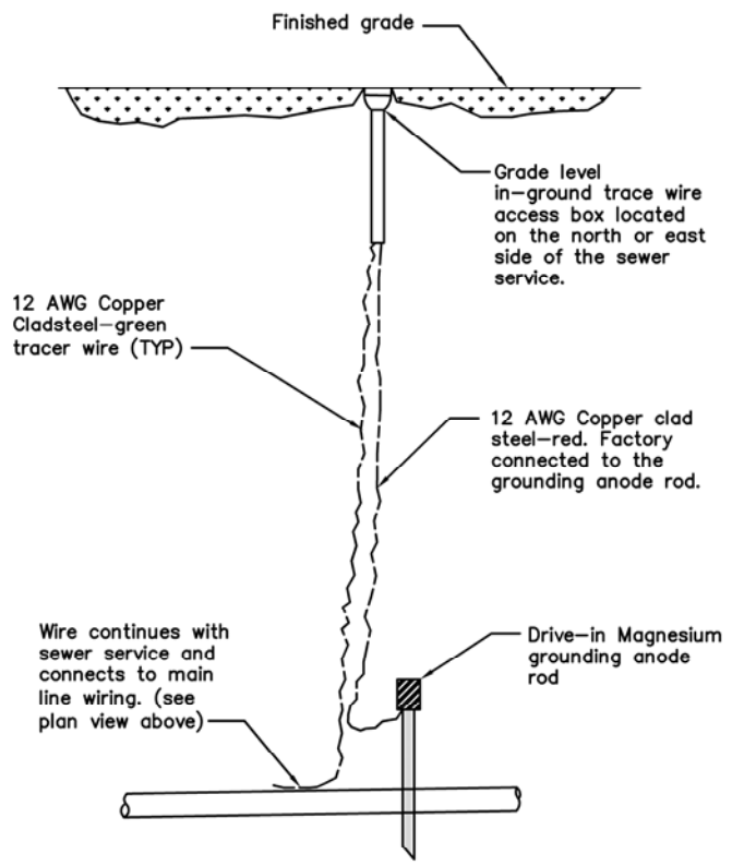
Sanitary Service-Section View Not to scale
