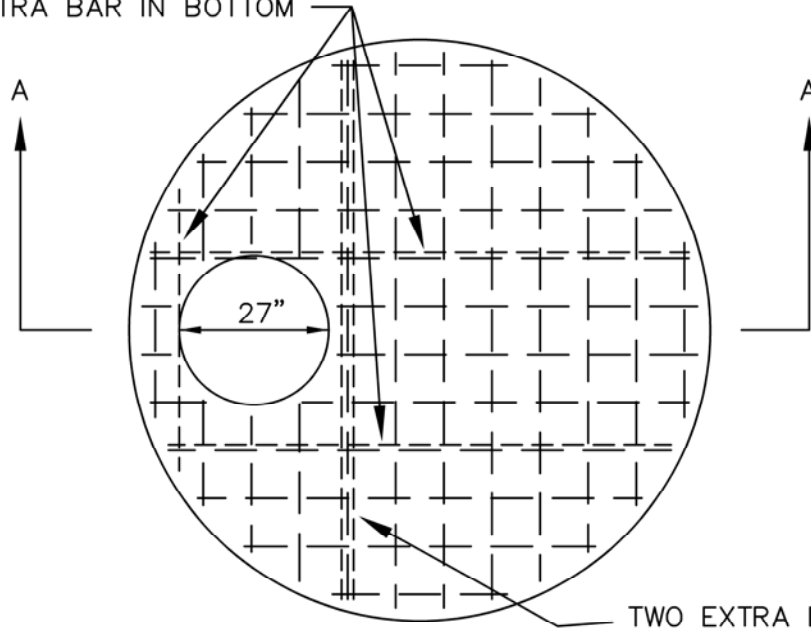
PLAN OF COVER
